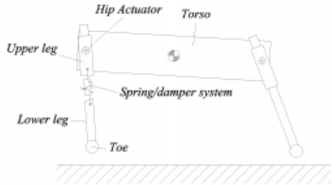
Figure 3. Scout II sagittal diagram
