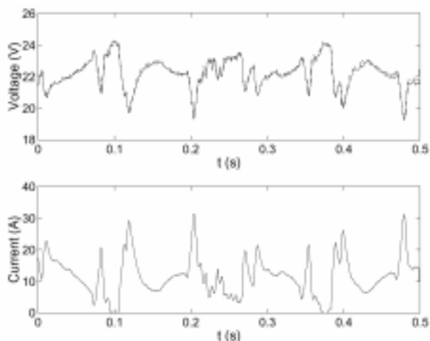
Figure 5: Battery voltage fluctuations (top, solid) as a function of load current (bottom). The top graph shows both the measured battery voltage (solid) and the battery voltage estimation (dash) based on an internal resistance model. The exceptionally good match between experimental and model data validates the simple internal resistance model (24V nom. Battery voltage with 0.15 Ohms internal resistance, and motor data taken from data sheet).
