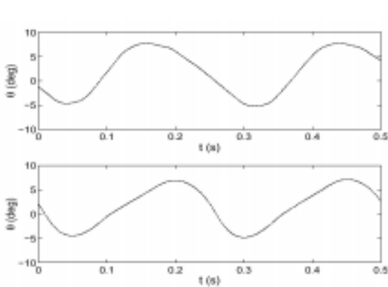
Figure 7: Body angle. Experiment (top), simulation (bottom)
