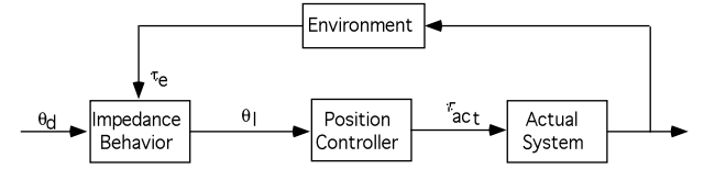
Fig. 2. Schematic of Position-based Impedance Control.
