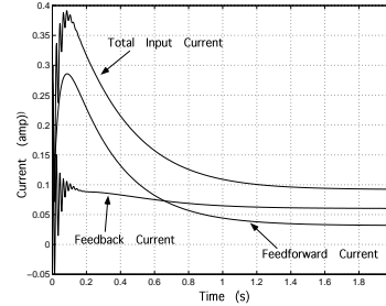
Fig. 6. Current Inputs for Z_d=1.6 .
