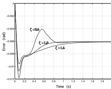
Fig. 5. Error vs Time for Z_d=0.6, 1.0 and 1.6 .
