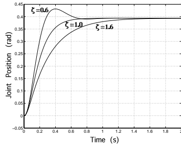
Fig. 4. Step Response for Z_d=0.6, 1.0, \& 1.6 .
